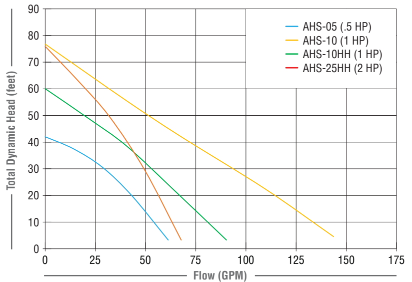
AHS Series Family Curve
