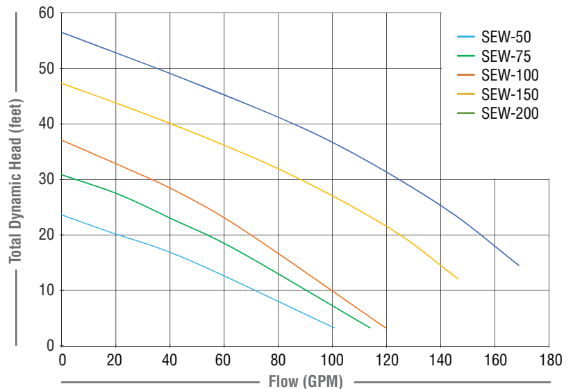
SEW-2" Solids Series Family Curve
