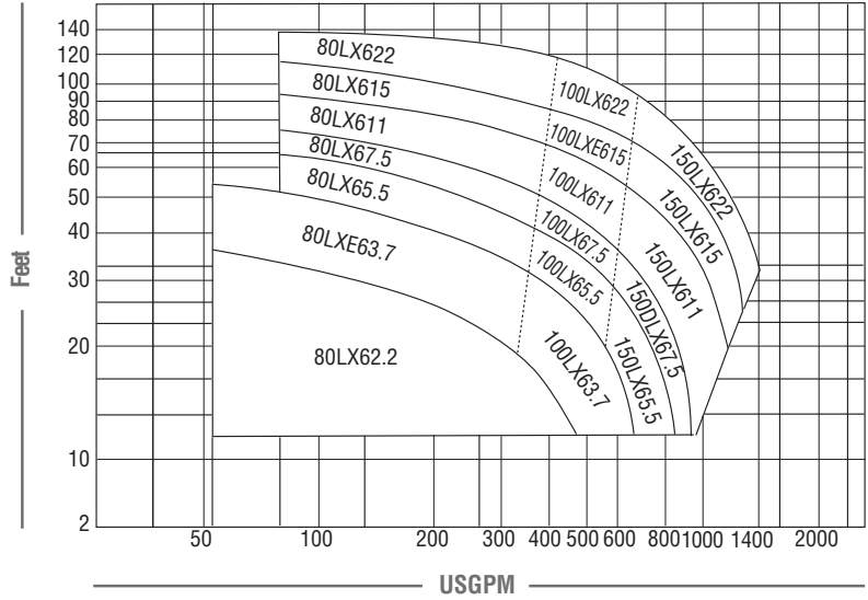
LX Series Family Curve
