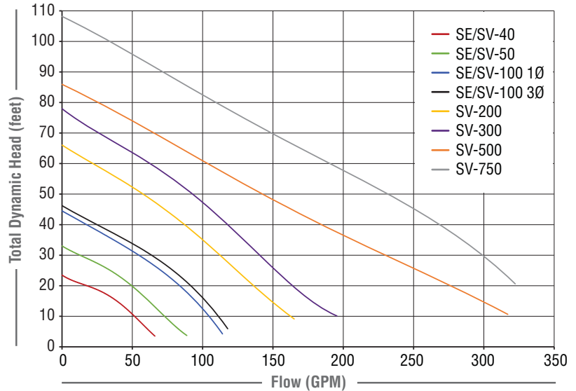
SV/SE Series Family Curve
