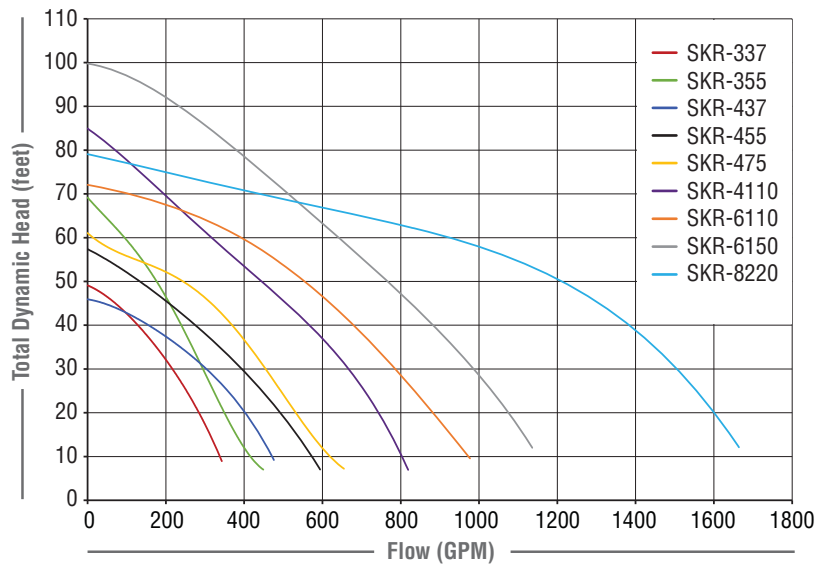
SKR Series Performance Curve
