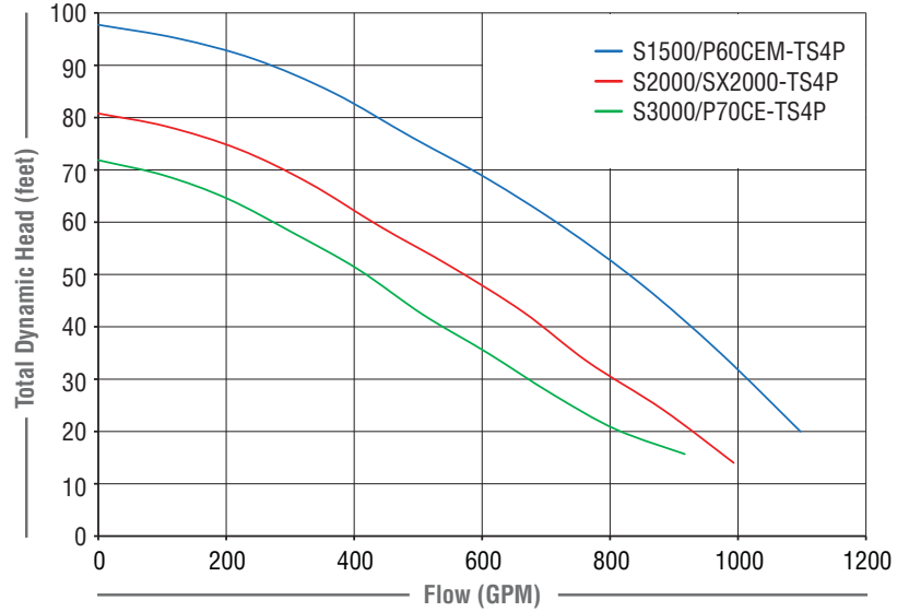
S-Series Solids Performance Curve
