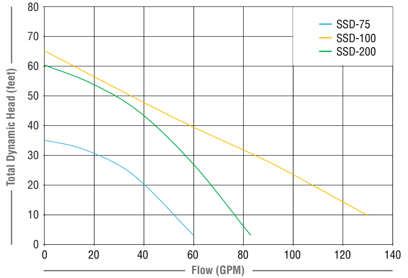
SSD Series Family Curve
