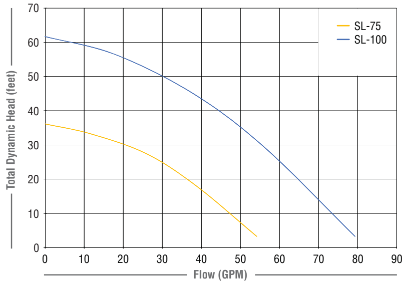
SL Series Family Curve
