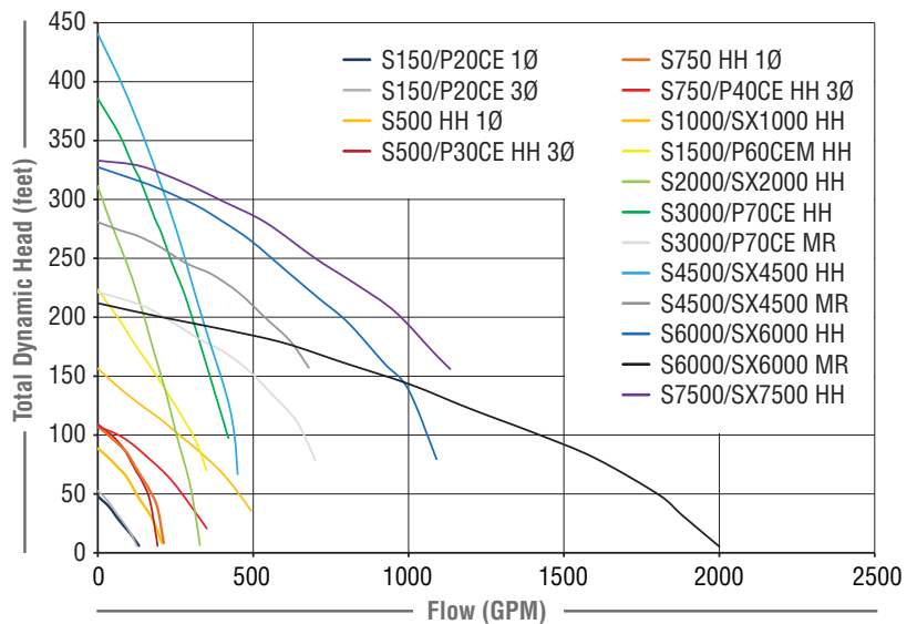
P- and S-Series HH Family Curve
