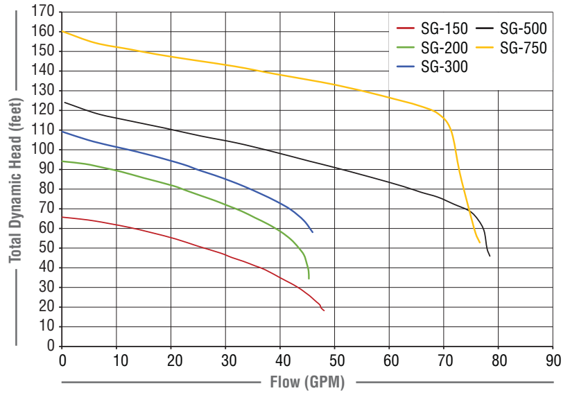
SG Series Family Curve
