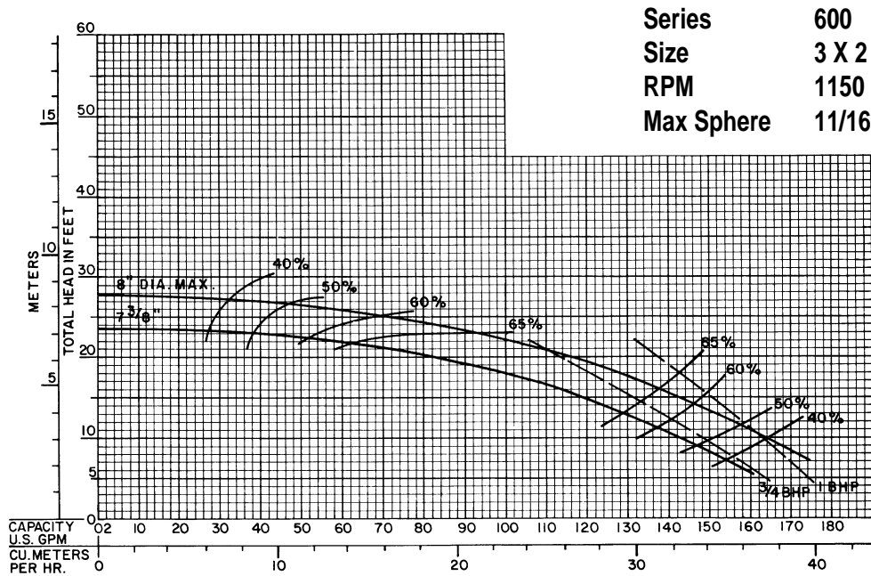
Curve DS-1620
