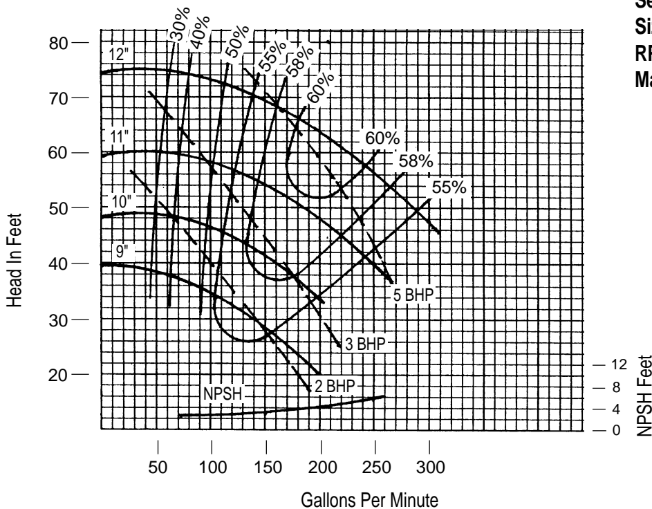
Curve LL-1916
